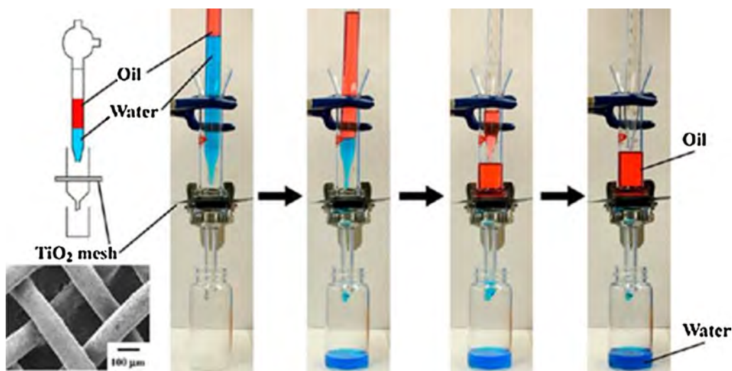
Fig. 29. Oil–water separating device based on titanium mesh, n -hexadecane dyed with Sudan IV (red) and water dyed with methylene blue (blue) were used as oil and water phases, respectively. (For interpretation of the references to color in this figure legend, the reader is referred to the web version of this article.) (Reprinted from Langmuir 29 (2013) 6784–6789 with permission from American Chemical Society).
